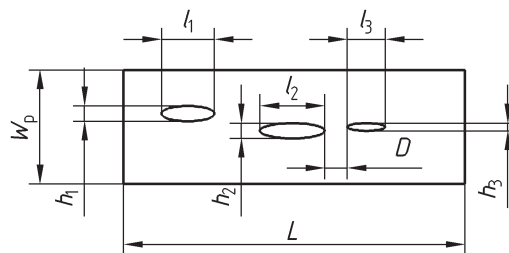
Figure C.6 — Elongated cavities and wormholes, D < l_3
