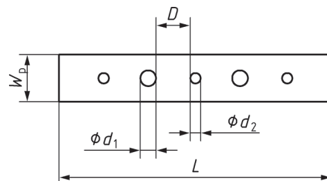
Figure C.3 — Linear porosity, D > d_2
