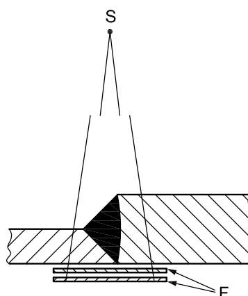
Figure 19 — Multi-film technique
