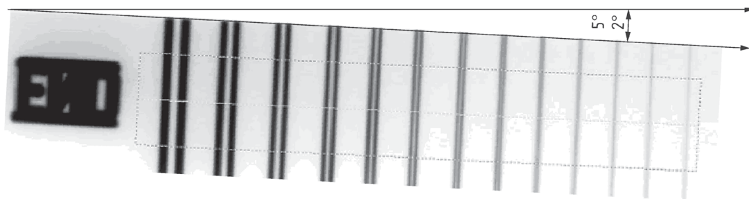
a) Image of the duplex wire IQI as shown in a radiograph
