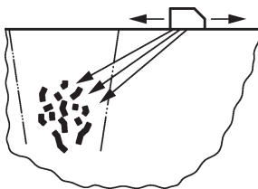
a) Probe position of A-scan and variation in signal amplitude
