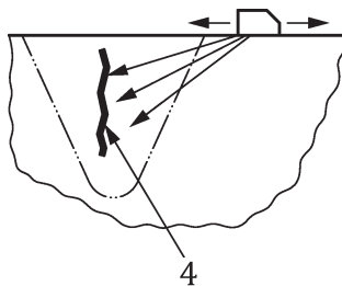
a) Probe position of A-scan and variation in signal amplitude
